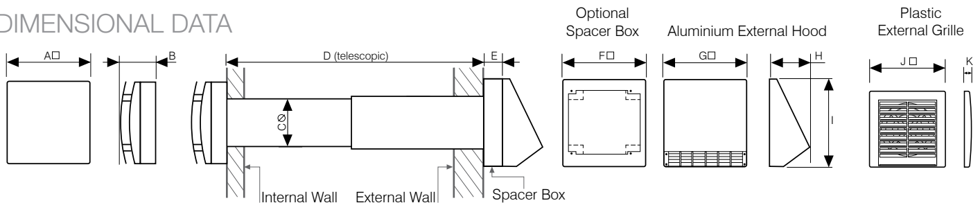
Spacer Box 190mm. For walls 110mm to 240mm thick.
